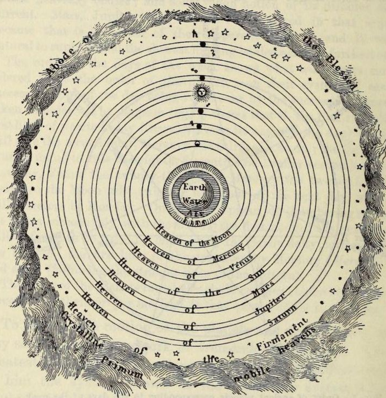
FIG. 8.—Ptolemaic system.
